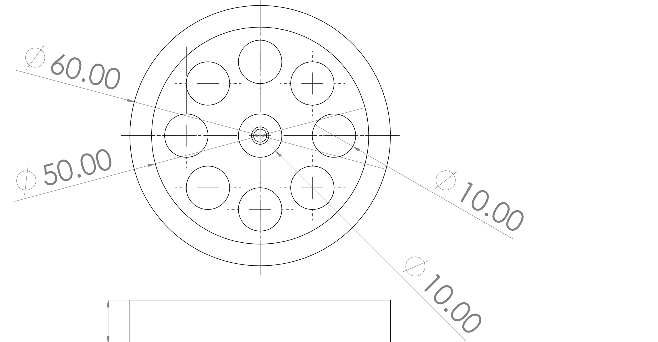
Flywheel
