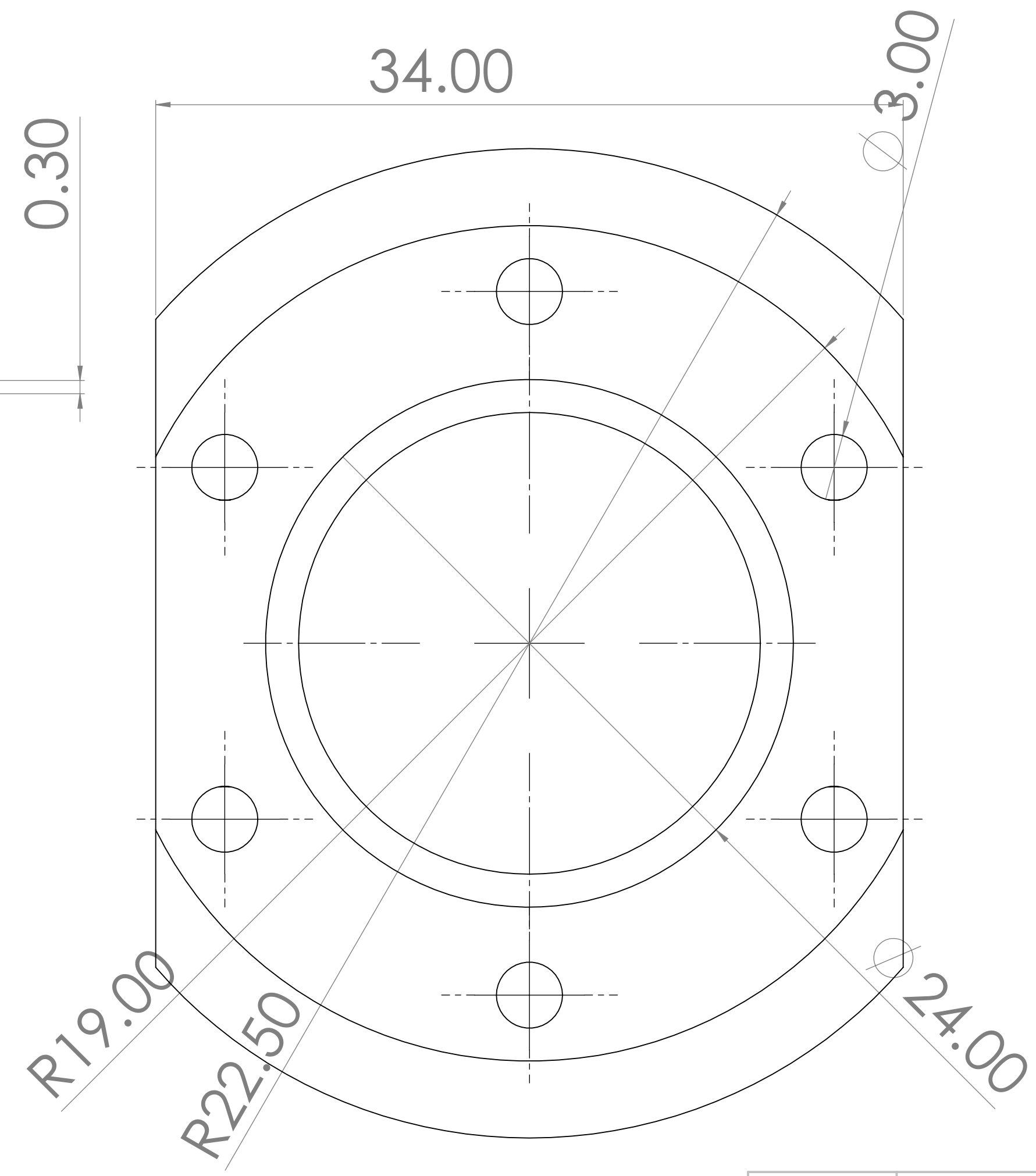
Cylinder
